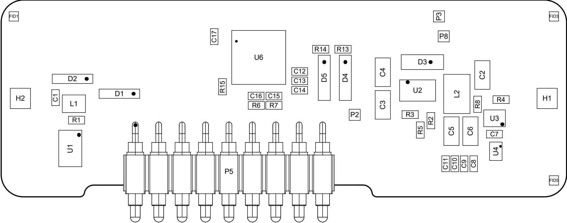
View from Top side (Scale 4:1)
